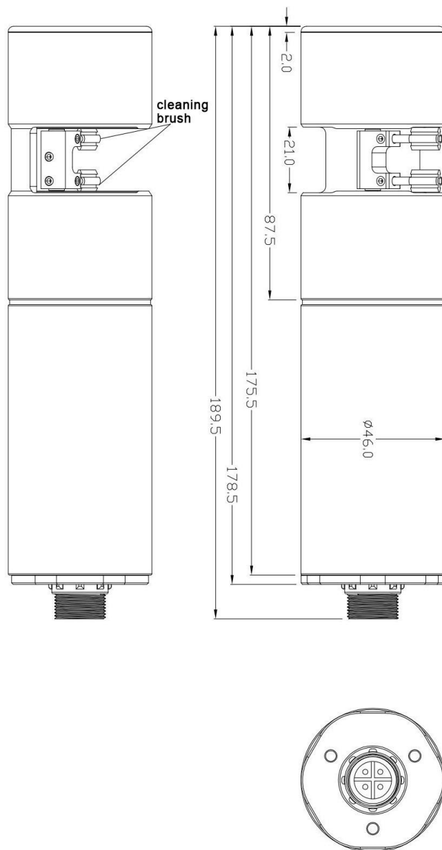
▲ Y531-A self-cleaning color sensor size
